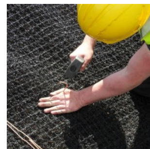
Fig 4: Pin GeoMat to slope
